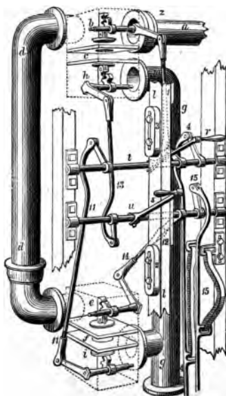
FIG. 82.—Valve-Gear of the Albion Mills Engine.
